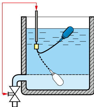
EMPTYING CONTROL
