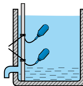
MULTI-LEVEL SWITCHING
