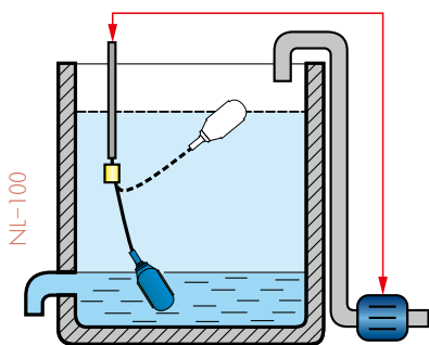
FILLING CONTROL
