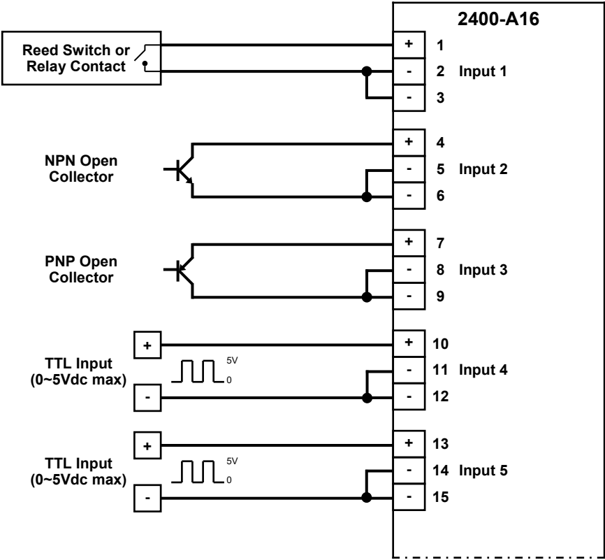
2400-A16 Input Connection Diagram Digital Signals Into Universal Inputs 1~16.
