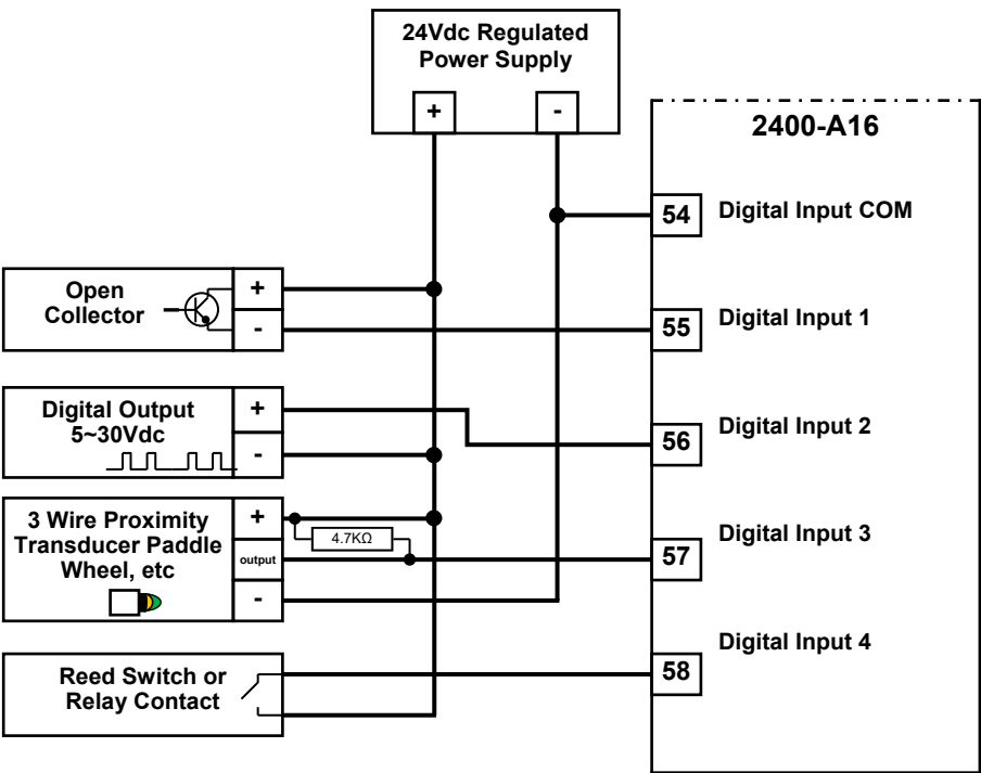
2400-A16 Input Connection Diagram for Digital Signals Into Dedicated Digital Inputs 54~58.
