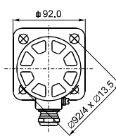
Rectangular connection flange
