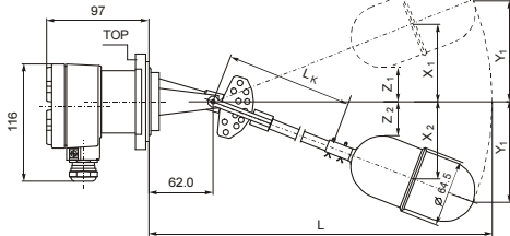
MKA-220 Adjustable switch differential, vertical mounting
