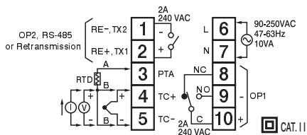
Figure 2.5 Rear Terminal Connection for C91
